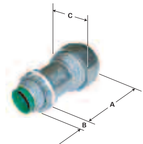
Connector Dimensions
